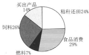
图 5 2000 年收获物氮素分配 (总氮 4 325 kg) Figure 5 N distribution of products in the year 2000 (Total N: 4 325kg)
