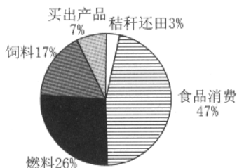
图 6 60 年代收获物氮素分配 (总氮 1 172 kg) Figure 6 N distribution of products in the years 1960s (total N: 1 172 kg)
